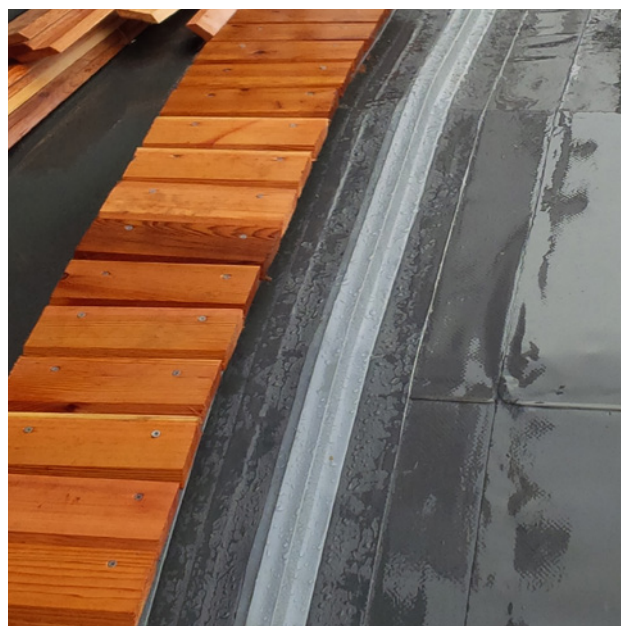
Wooden slats are secured to RENOLIT ALKORPLAN Solar profiles.
