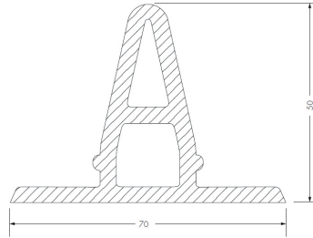
RENOLIT ALKORDESIGN profile X-Large
