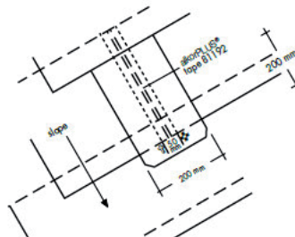
Figure B: Aluminium foil tape and non-glued area
