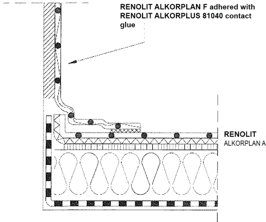
Bonded edge detail and upstand
